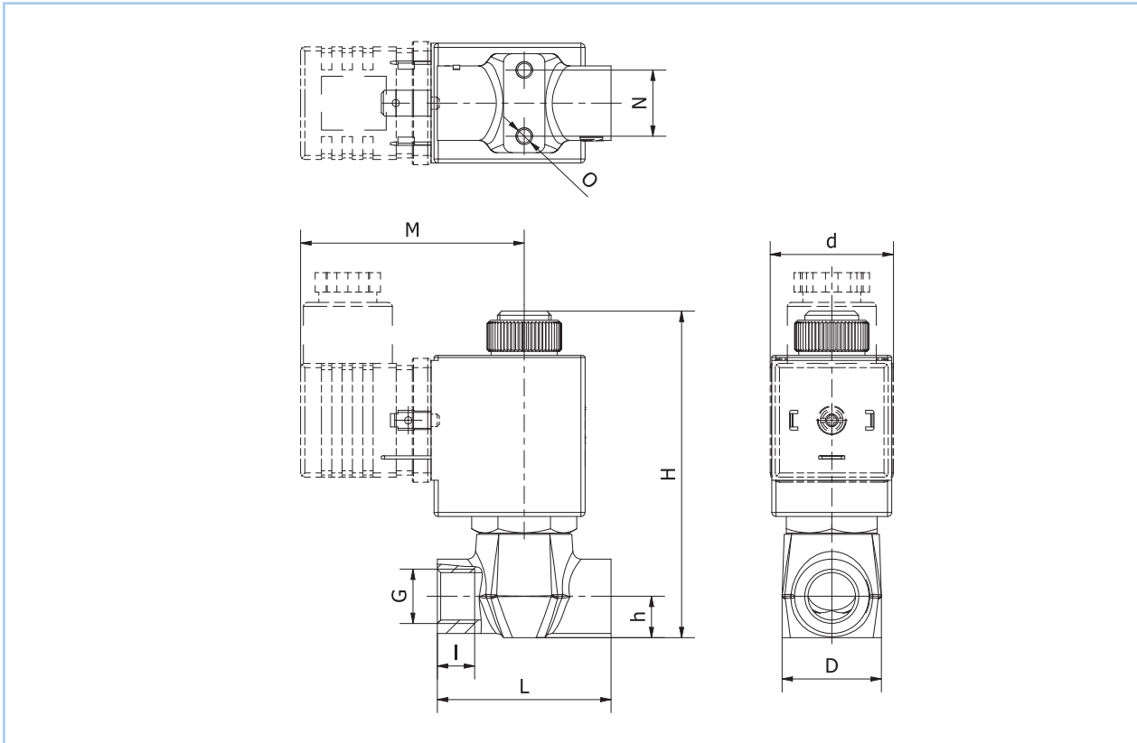
Dimension table for type 20 in mm, approx. weight in g
